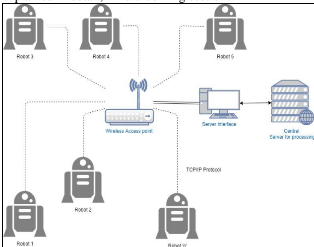
Fig-5: Network architecture of entire system
