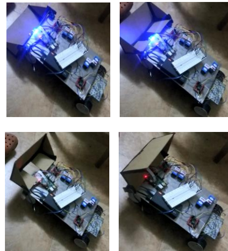
Fig-12: Actuation of tray in progress
