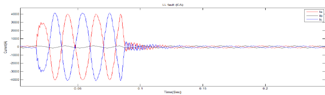
Fig. 7. LLL Fault at phase A, B & C with fault resistance 25 Ω
