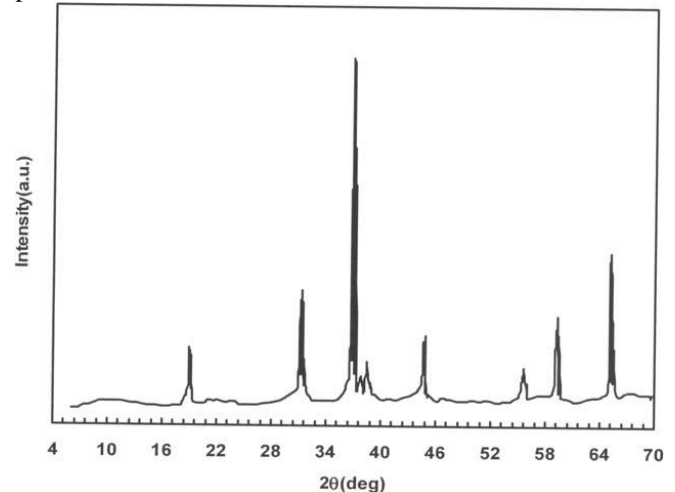
Figure 2 XRD of cobalt oxide nanoparticles.
