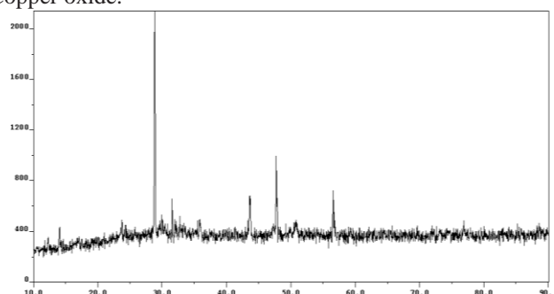
Figure 4 XRD of Iron / Copper oxide nanoparticles.
