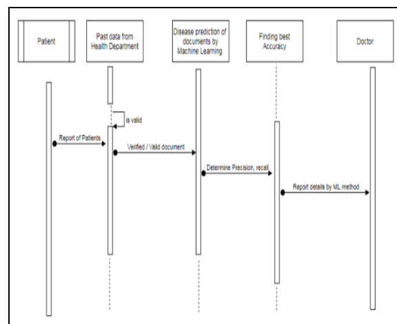
Fig 4: Dynamic work flow of sequence followed
