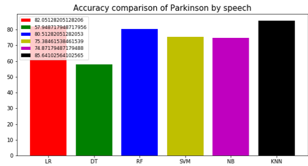
Fig 7: Accuracy based on speech Parameter
