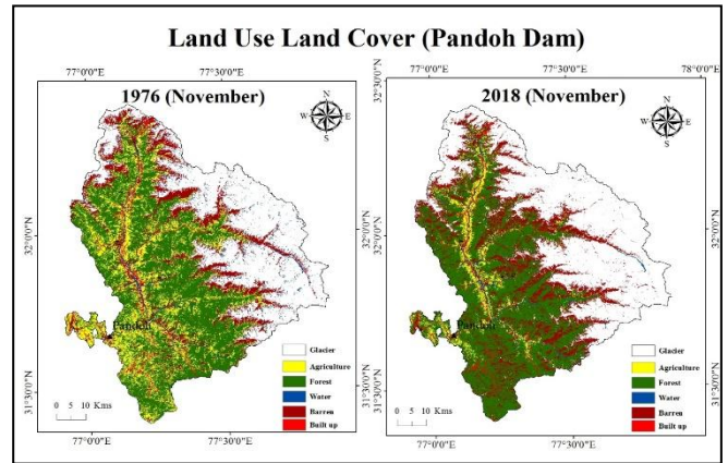
Fig.4. LULC for Pandoh (Lean Period)
