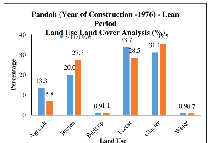
Fig.5. LULC area in % for Pandoh (Lean Period)
