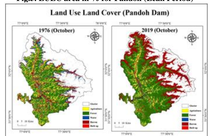
Fig.6. LULC for Pandoh (High Flow Period)
