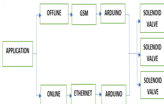
Figure 8: Block Diagram of Model
