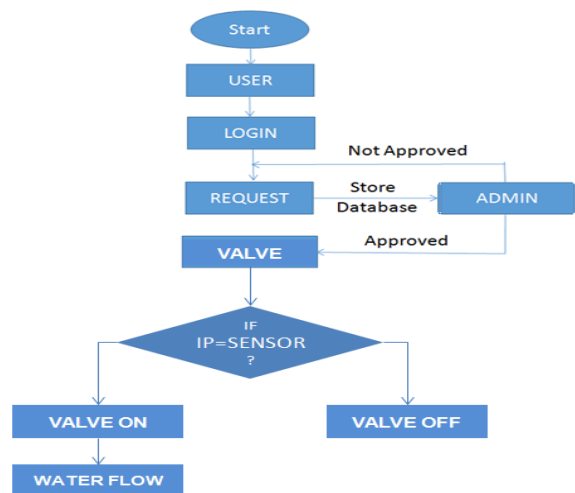
Figure 11: Flow Chart-Water Request and Delivery in Model
