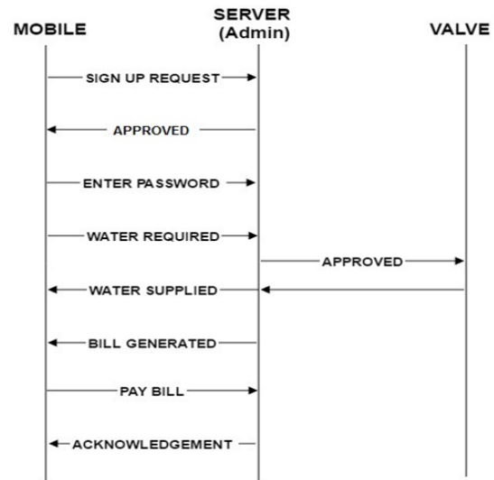
Figure 9: Sequence Diagram of Model
