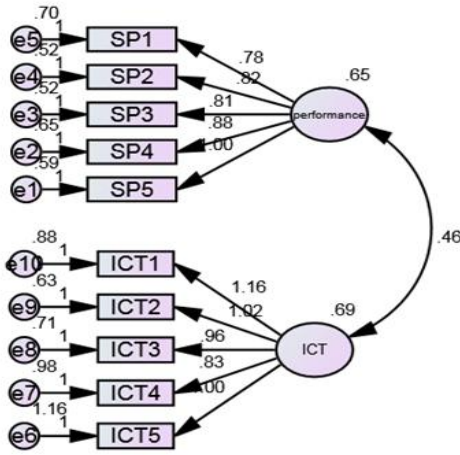
Diagram 1 Showing CFA analysis
