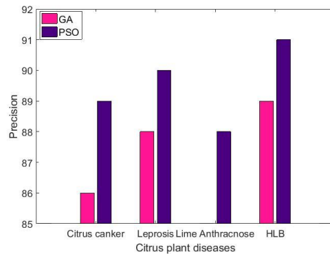
Fig. 2. Comparison of Precision
