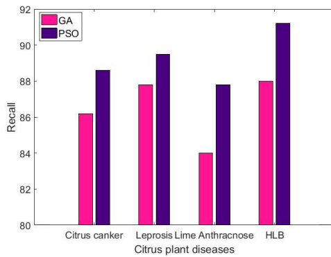
Fig. 3. Comparison of Recall
