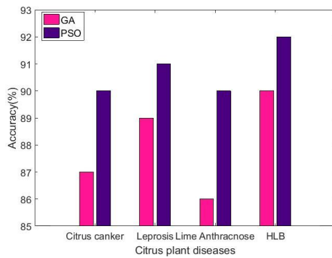
Fig. 1. Comparison of Accuracy
