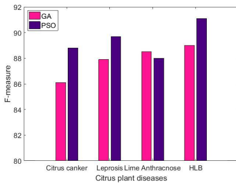
Fig. 4. Comparison of F-measure
