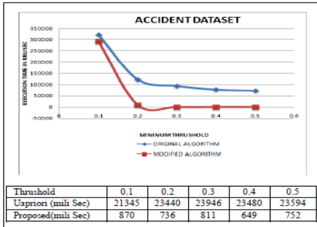
Fig. 7. Execution of Uapriori and Proposed algorithm on Accident dataset
