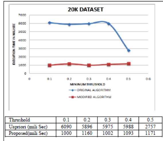
Fig. 1. Execution of Uapriori and Proposed algorithm on 20K dataset
