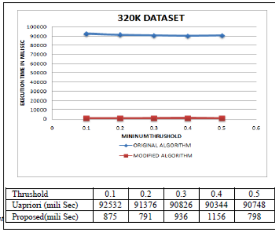
Fig. 5. Execution of Uapriori and Proposed algorithm on Gazelle dataset
