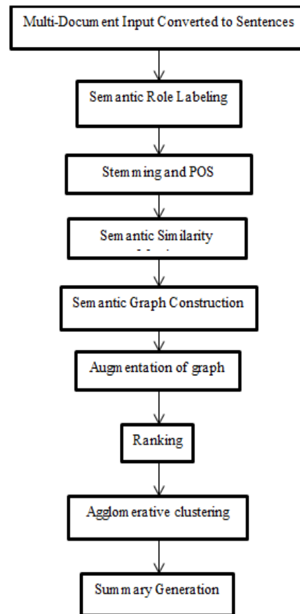
Figure 1: Block Diagram of the System Developed Jiang(C1, C2) = IC(C1) + IC(C2) - 2 * IC(Iso(C1, C2)) (1)
