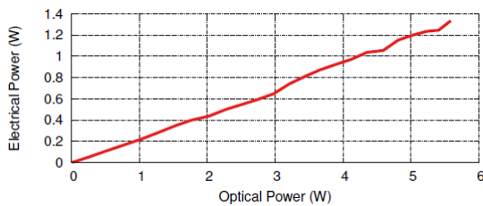
Fig. 6 PV cell efficiency
