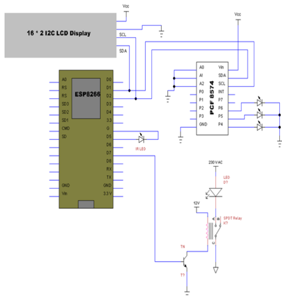
Fig. 2 Circuit diagram of Transmitter
