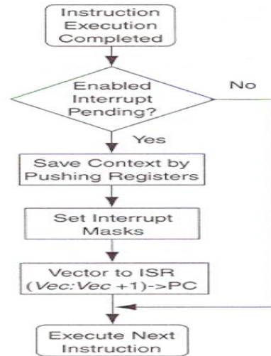
Fig. 5 System Flowchart
