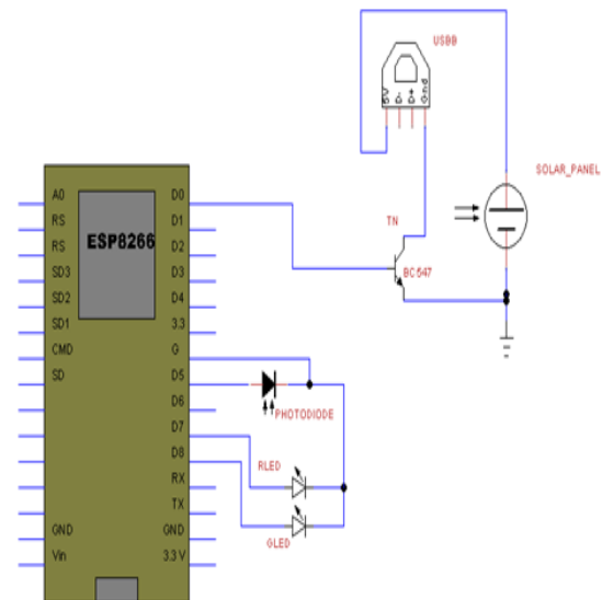
Fig. 3 Circuit diagram of Receiver
